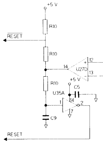
Figure B-17. 08116-66513: Reset circuit
