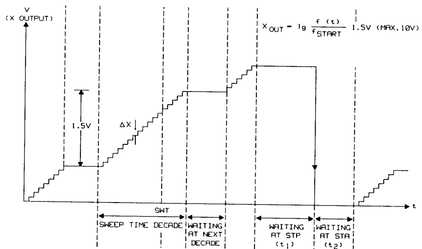
Figure 10.6-2. X-output in sweep mode
