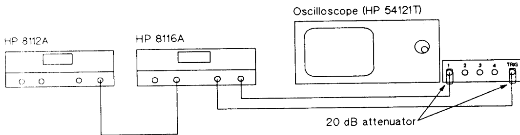
Figure 8-14. Amplitude Modulation Verification Test
