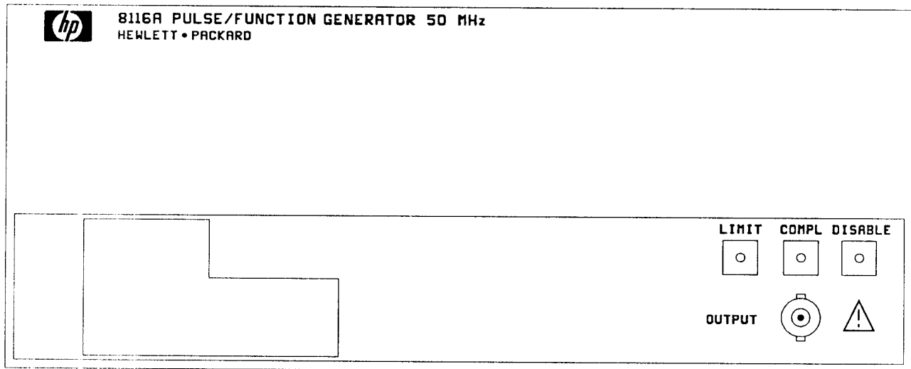
Figure 4-13. Output controls
