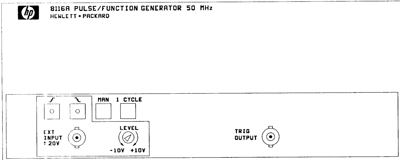
Figure 4-3. External Trigger Controls
