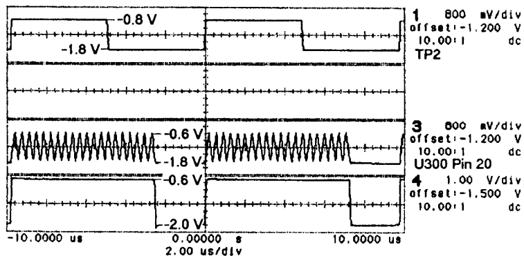
Figure 10.3-10. Width Generator Input and Output signals
