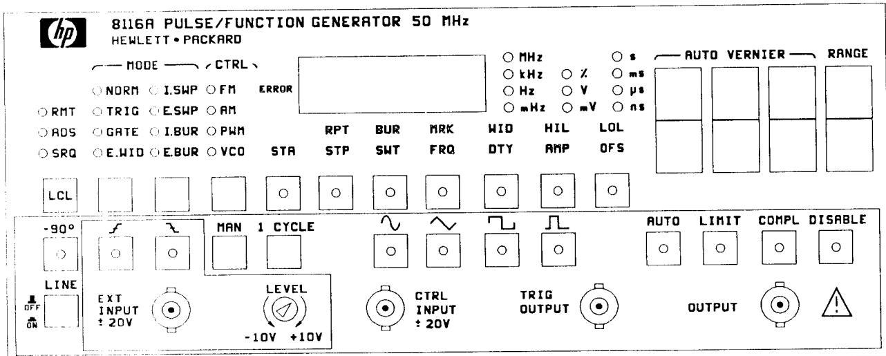
Figure 4-1. HP 8116A Front Panel
