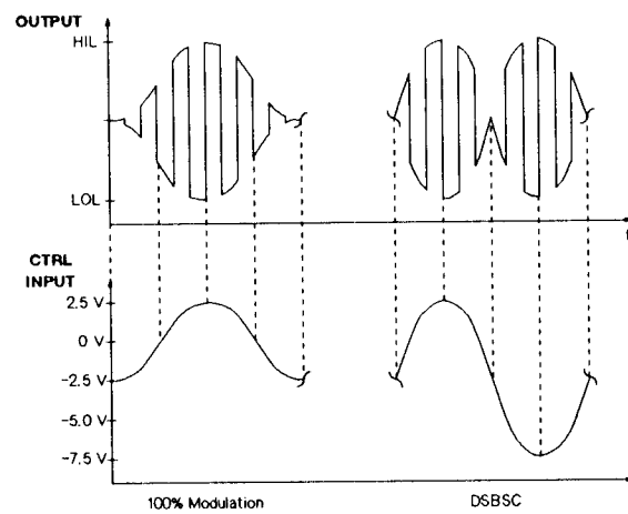
Figure 4-6. Amplitude Modulation
