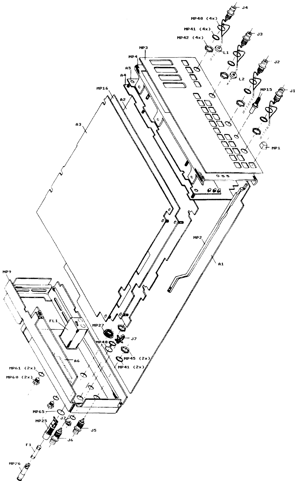
Figure B-26. Mechanical Parts - 2
