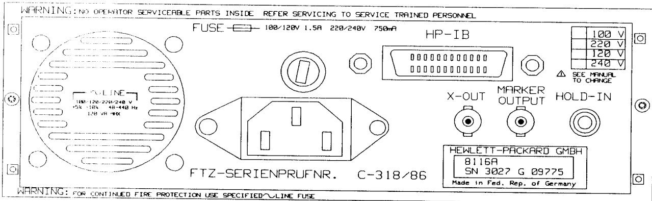
Figure 4-14. Rear panel
