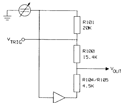
Figure 10.3-1. Simplified Trigger-level circuit
