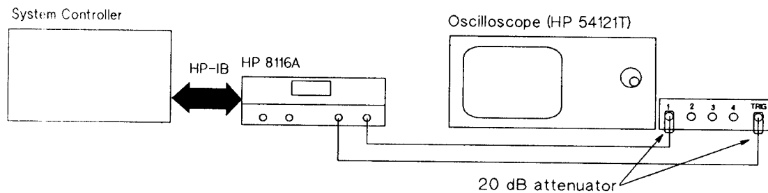
Figure 8-18. HP-IB Verification Test
