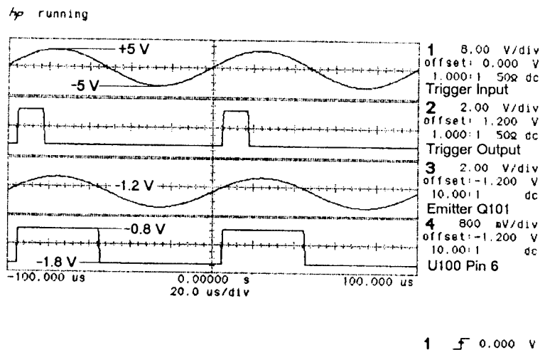
Figure 10.3-8. Trigger Input Amplifier signals
