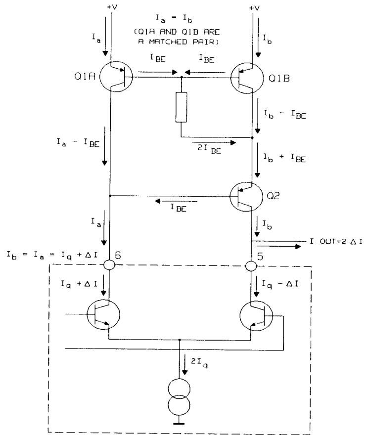
Figure 10.4-2. Current Mirror
