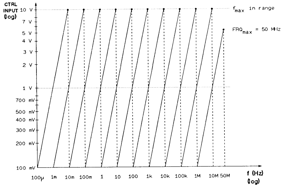
Figure 4-8. VCO characteristics
