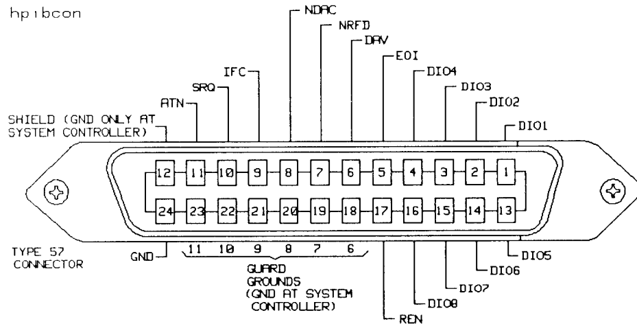
Figure 3-3. HB-IB Connector
