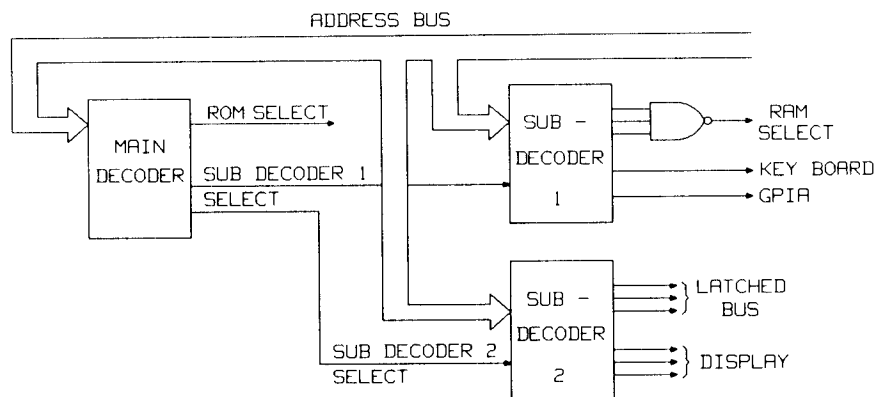
Figure 10.7-3. Address decoding
