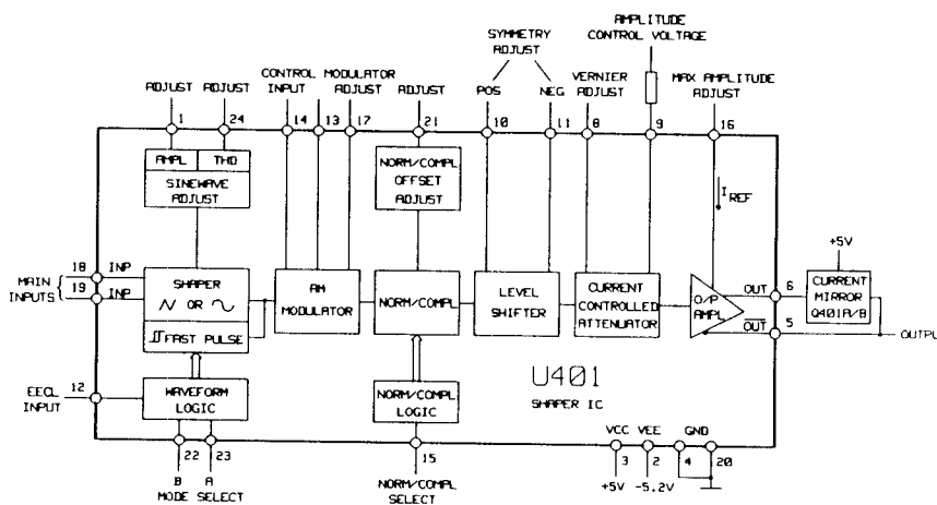
Figure 10.4-1. Shaper IC Block Diagram
