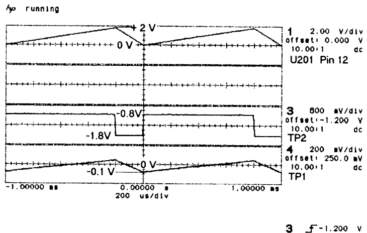
Figure 10.3-9. VCO Input and Output signals
