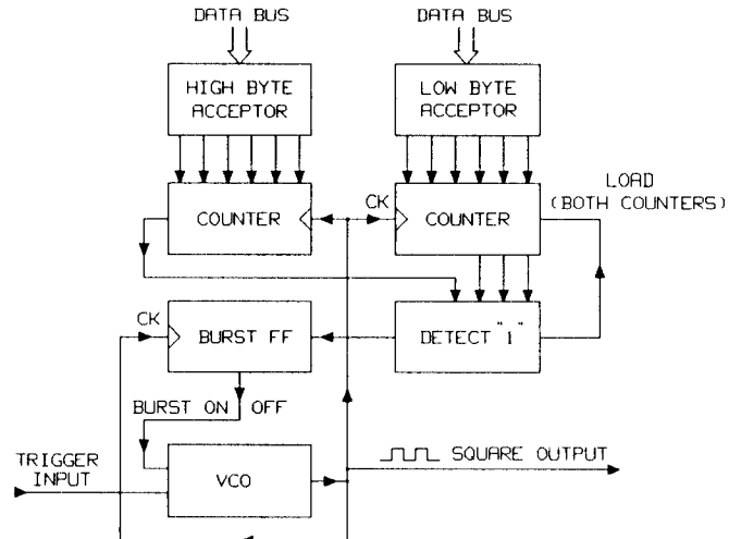
Figure 10.6-1. Simplified Burst Generator (Option 001)
