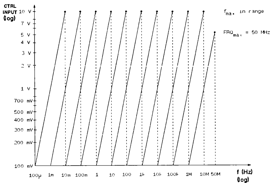
Figure 4-8. VCO characteristics
