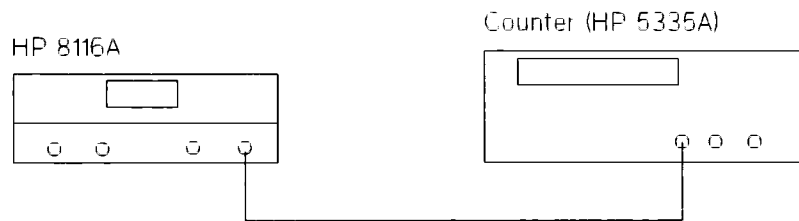
Figure 8-2. Duty Cycle Performance Test
