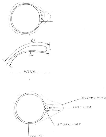
Fig. 4 - Wing profile & Collector positioning options
